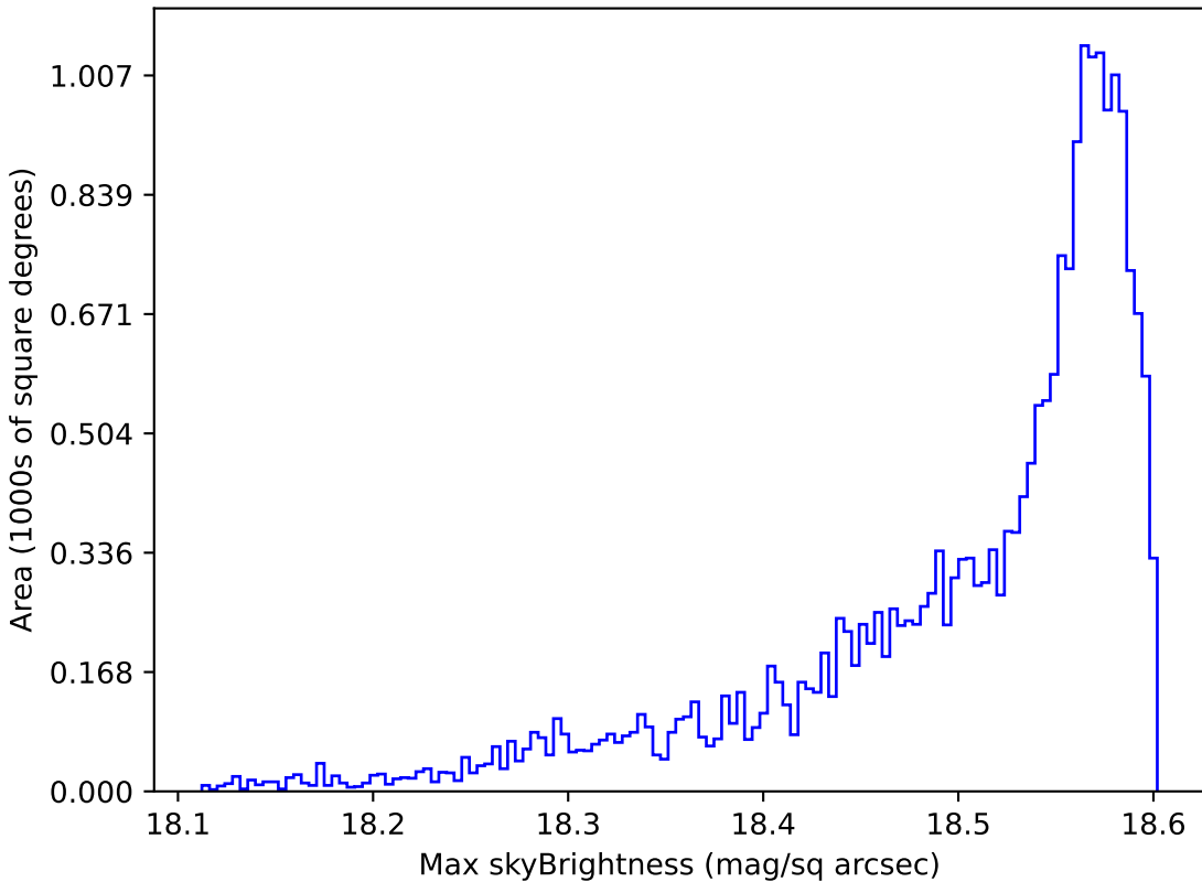
too_100_1v3.4_10yrs All sky y band: Max skyBrightness
