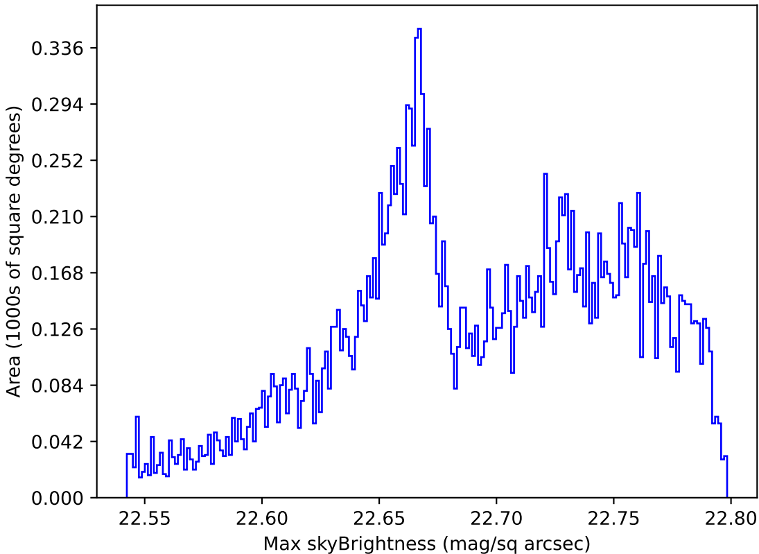
too_100_1v3.4_10yrs All sky u band: Max skyBrightness
