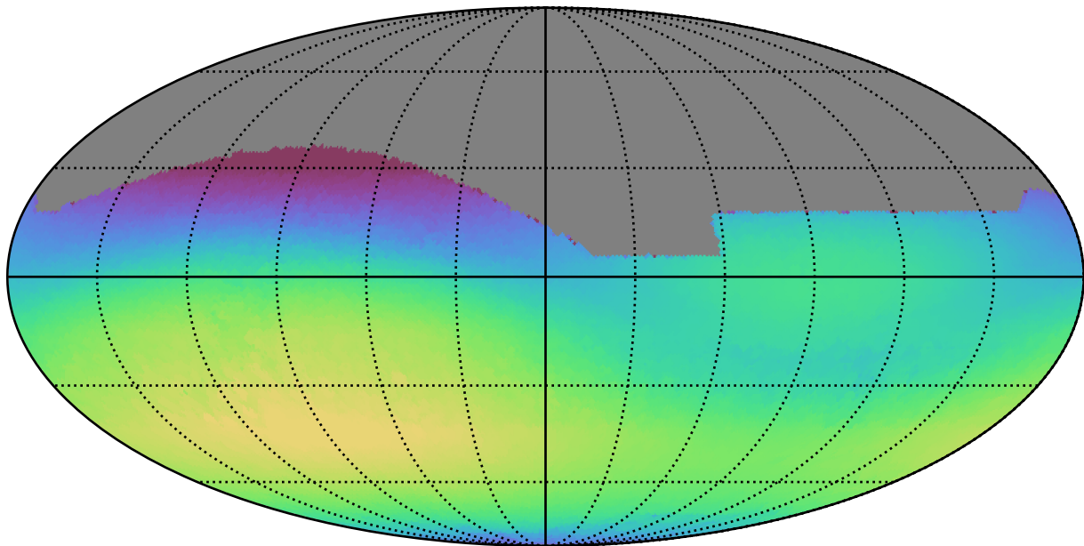
too_100_1v3.4_10yrs All sky r band: Max skyBrightness
