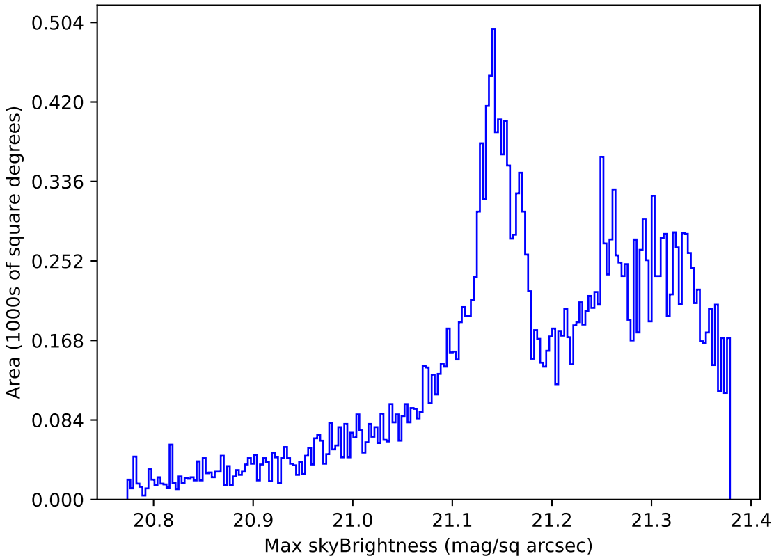
too_100_1v3.4_10yrs All sky r band: Max skyBrightness
