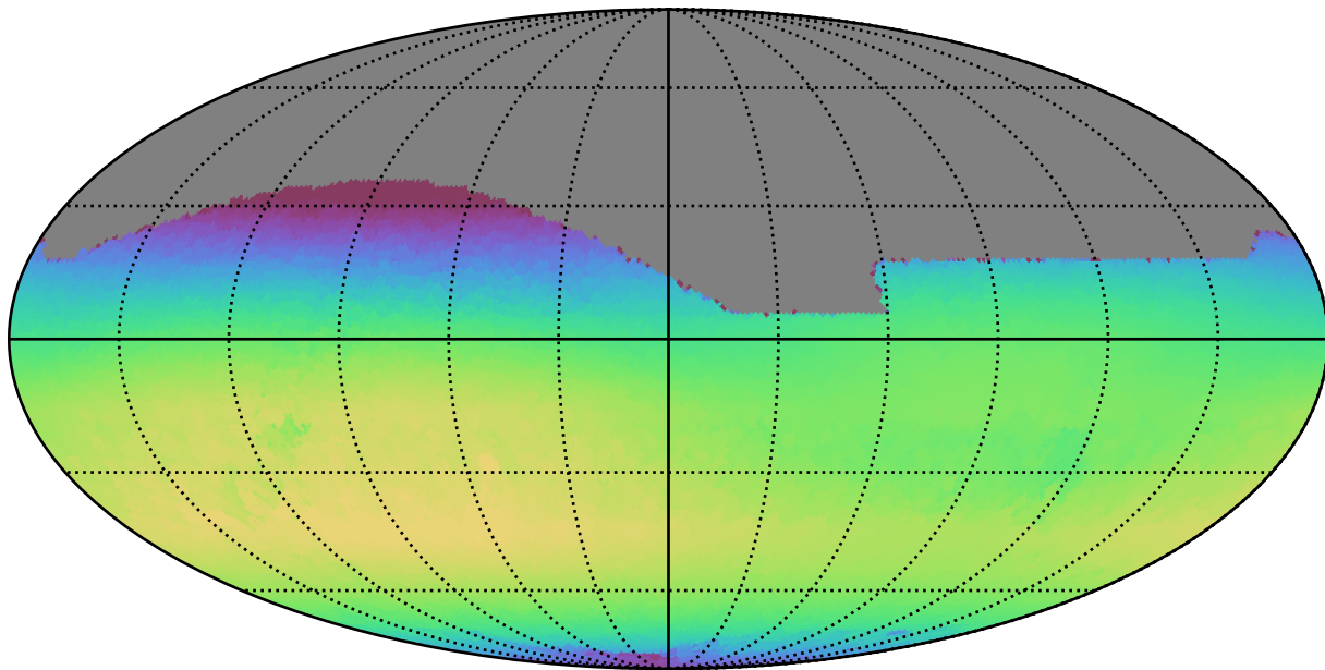
too_100_1v3.4_10yrs All sky i band: Max skyBrightness
