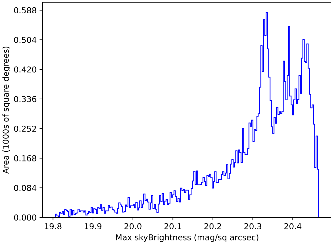
too_100_1v3.4_10yrs All sky i band: Max skyBrightness
