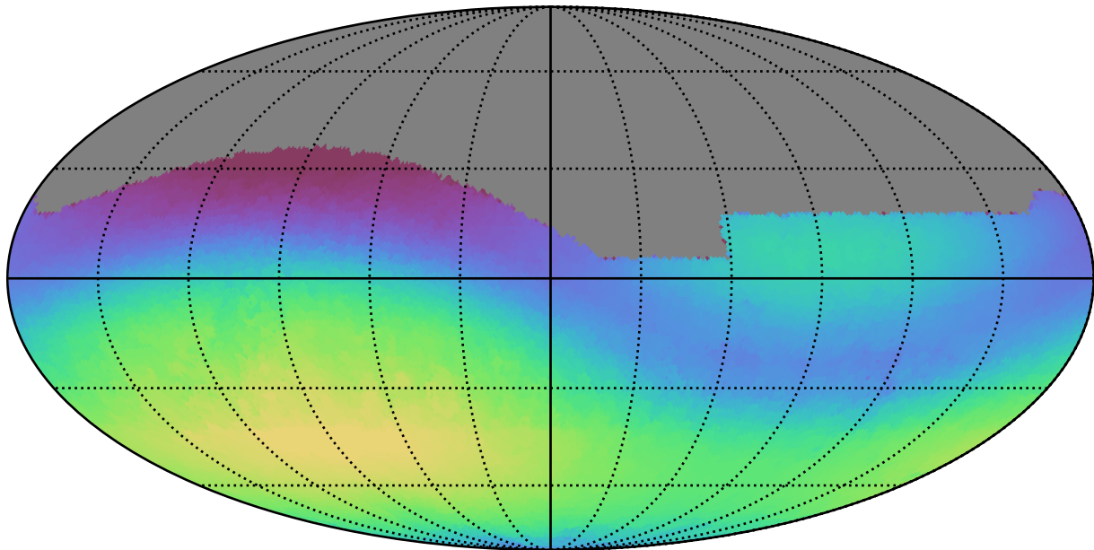
too_100_1v3.4_10yrs All sky g band: Max skyBrightness
