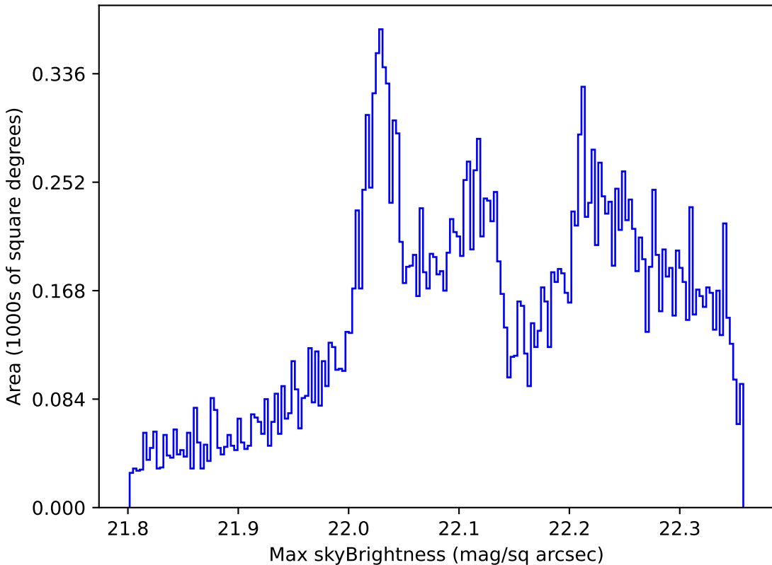
too_100_1v3.4_10yrs All sky g band: Max skyBrightness
