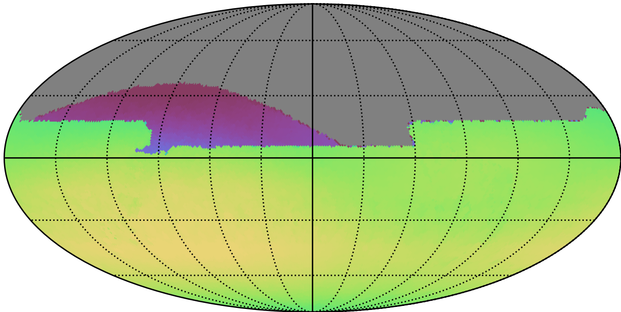
too_100_1v3.4_10yrs All sky all bands: Max skyBrightness
