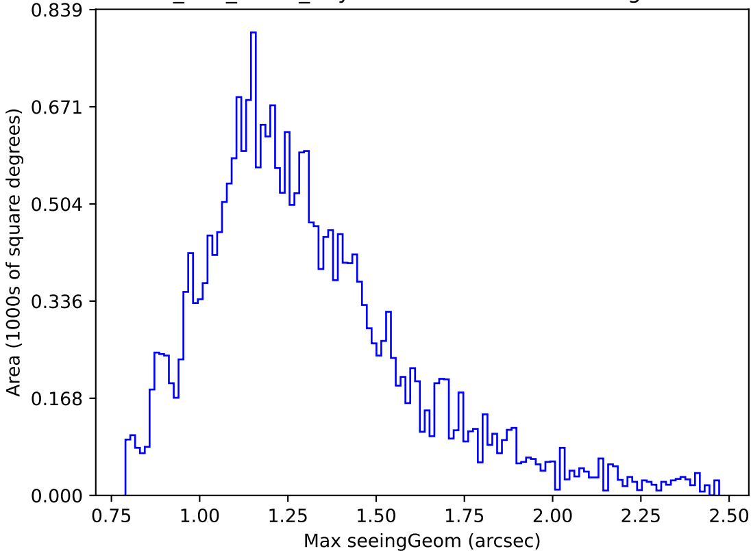
too_100_1v3.4_10yrs Yr 1 z band: Max seeingGeom
