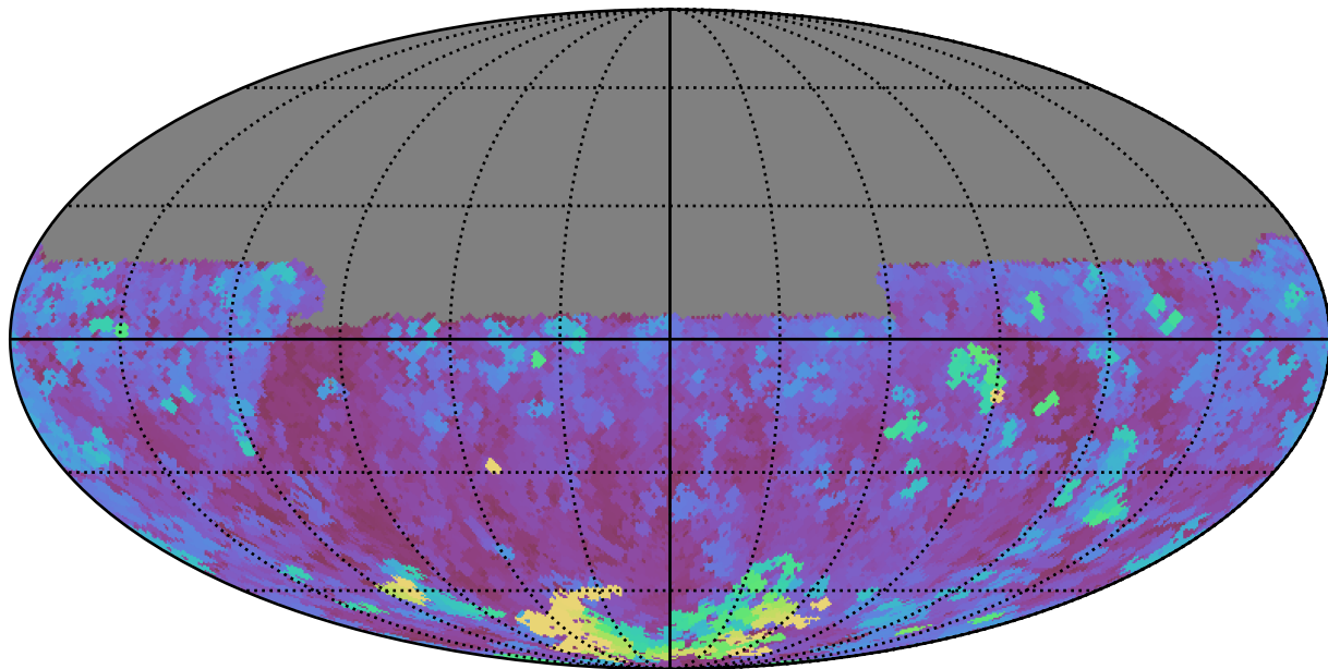
too_100_1v3.4_10yrs Yr 1 y band: Max seeingGeom
