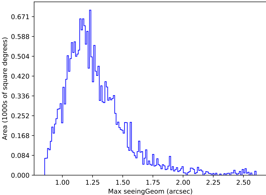
too_100_1v3.4_10yrs Yr 1 y band: Max seeingGeom
