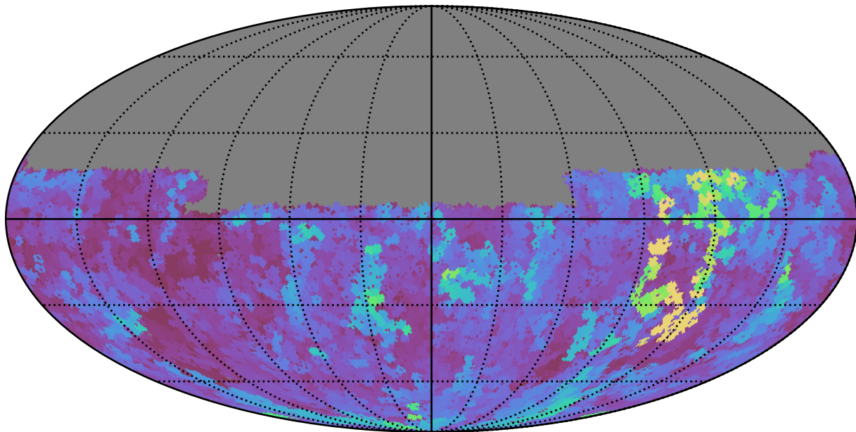
too_100_1v3.4_10yrs Yr 1 u band: Max seeingGeom
