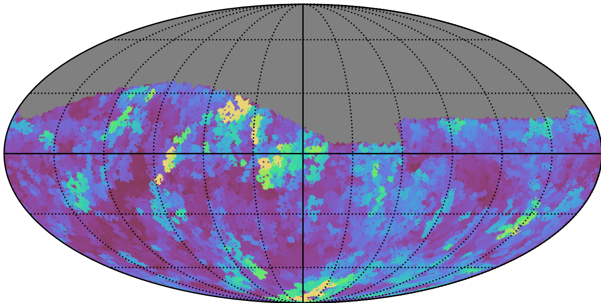
too_100_1v3.4_10yrs Yr 1 r band: Max seeingGeom
