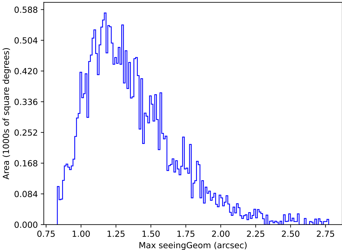
too_100_1v3.4_10yrs Yr 1 r band: Max seeingGeom
