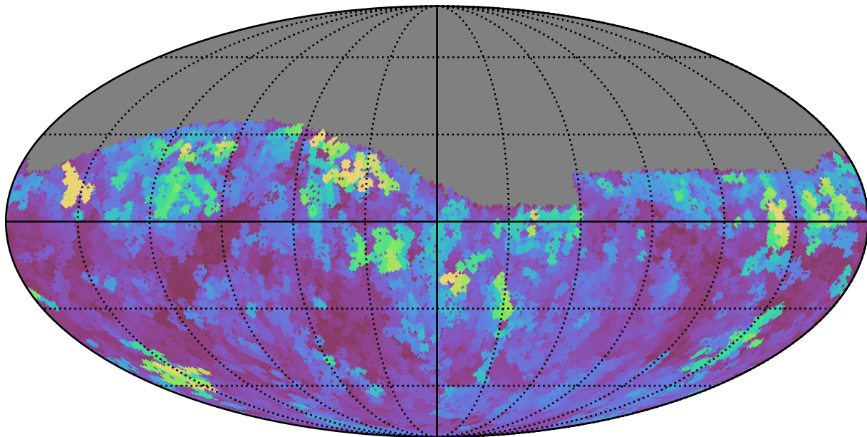
too_100_1v3.4_10yrs Yr 1 i band: Max seeingGeom
