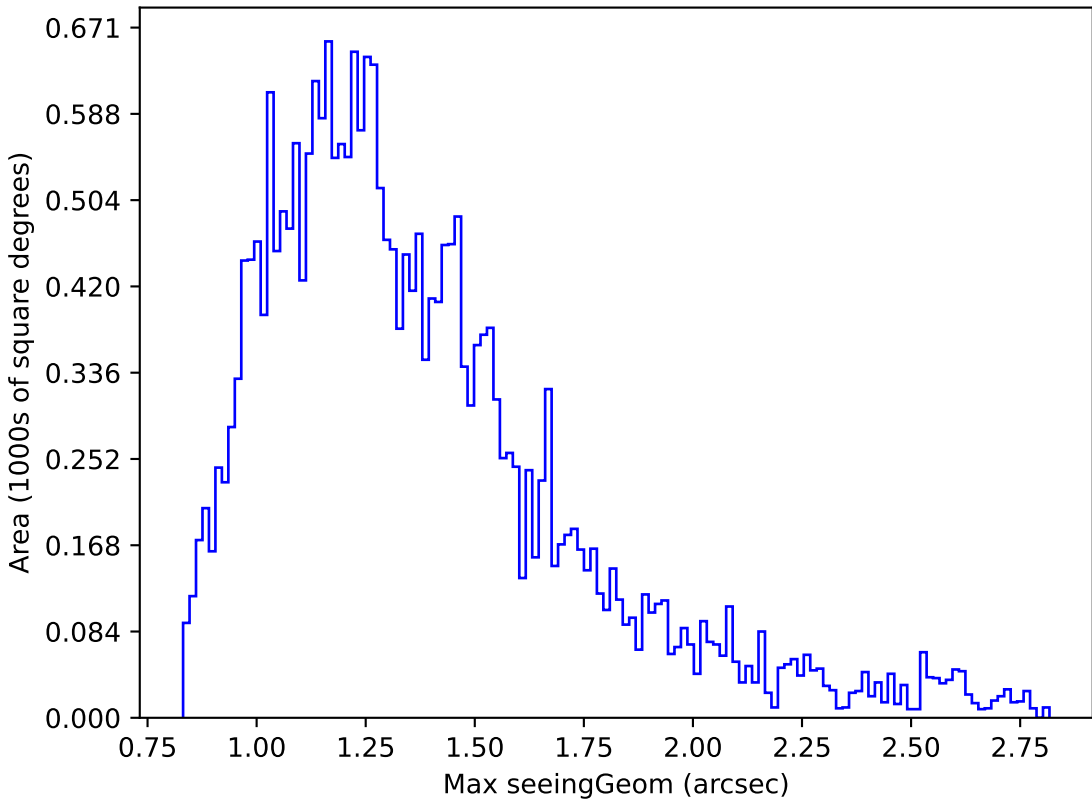
too_100_1v3.4_10yrs Yr 1 i band: Max seeingGeom
