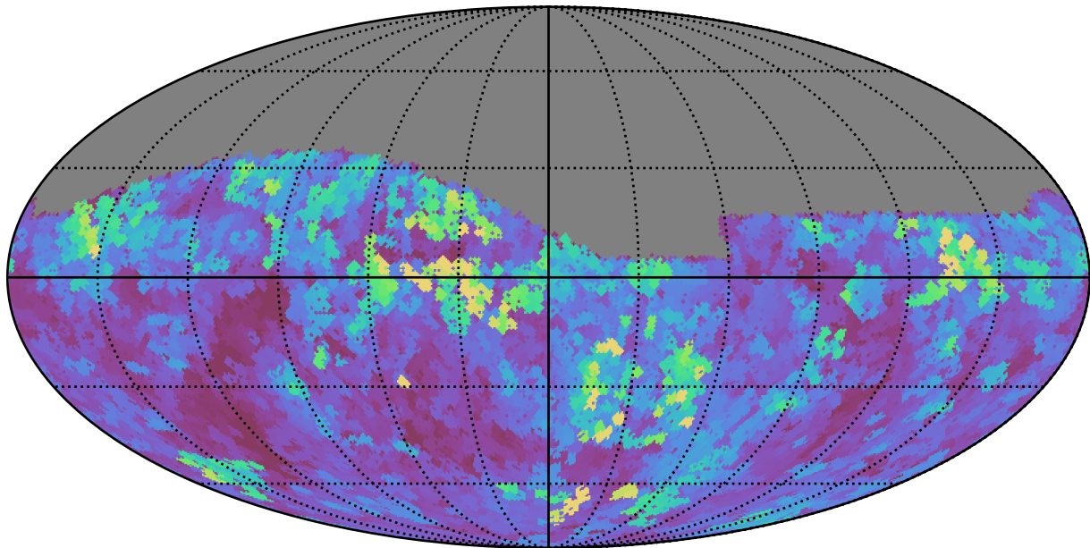
too_100_1v3.4_10yrs Yr 1 z band: Max seeingEff
