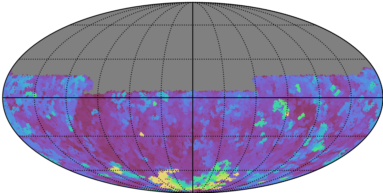
too_100_1v3.4_10yrs Yr 1 y band: Max seeingEff
