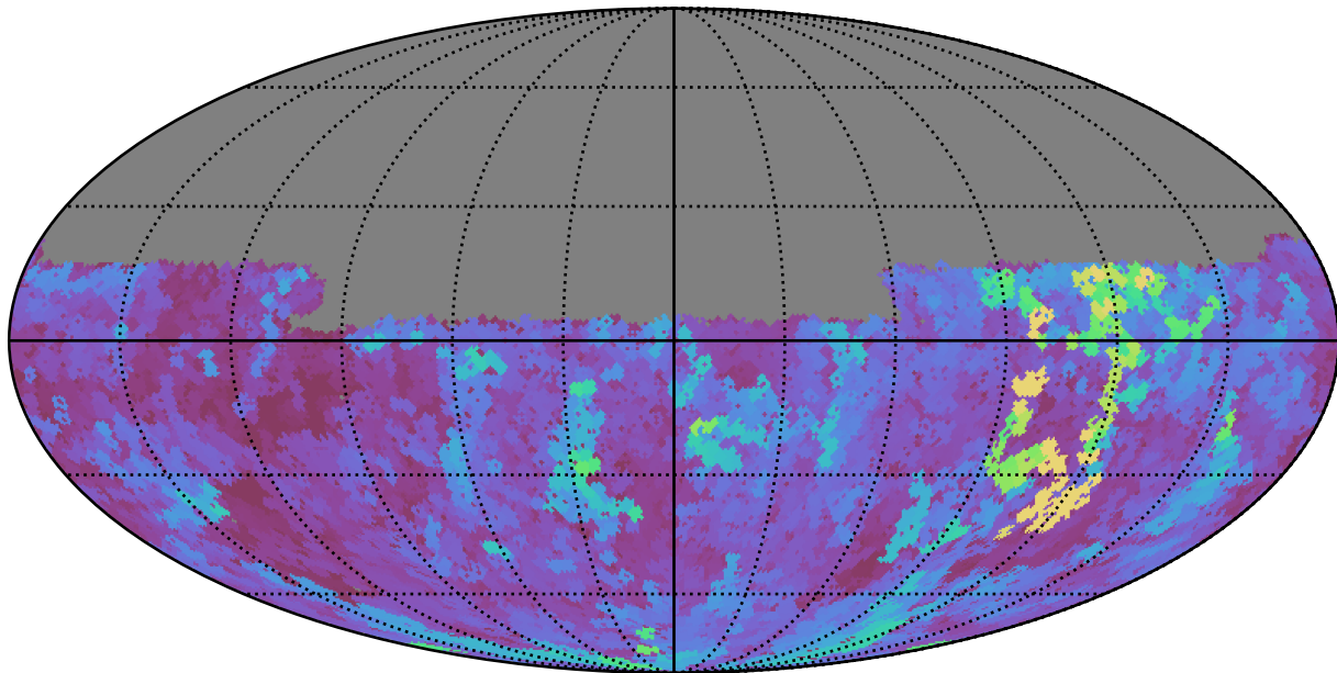
too_100_1v3.4_10yrs Yr 1 u band: Max seeingEff
