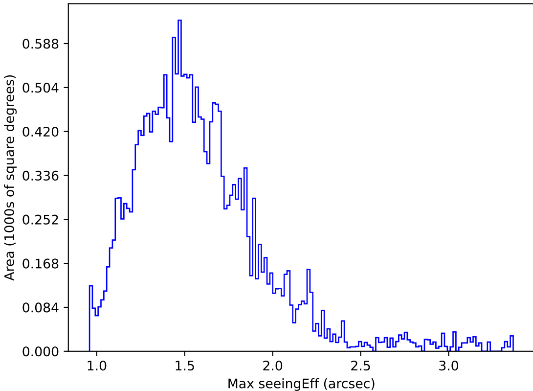
too_100_1v3.4_10yrs Yr 1 u band: Max seeingEff
