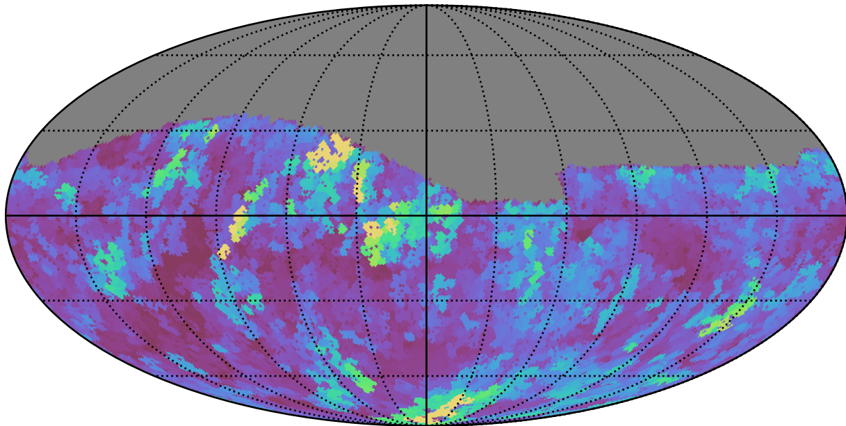
too_100_1v3.4_10yrs Yr 1 r band: Max seeingEff
