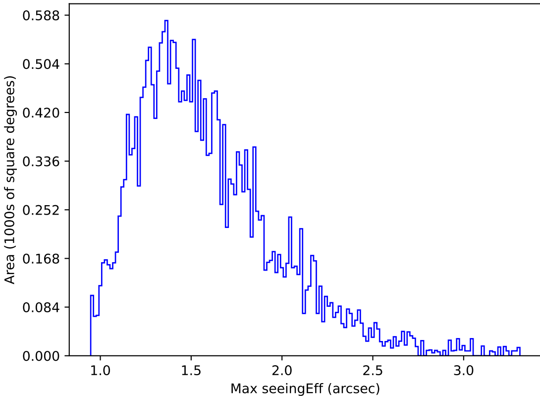
too_100_1v3.4_10yrs Yr 1 r band: Max seeingEff
