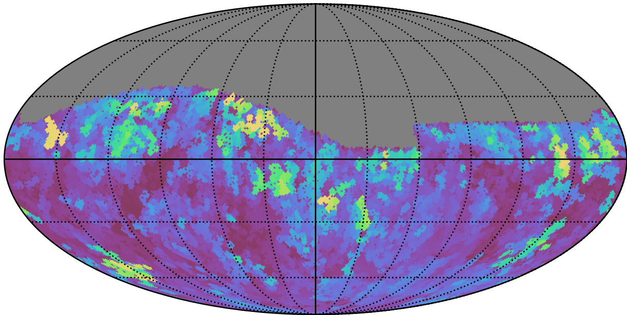
too_100_1v3.4_10yrs Yr 1 i band: Max seeingEff
