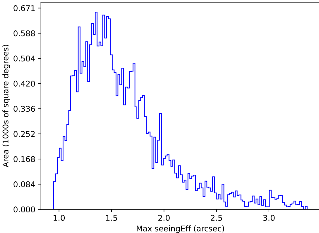
too_100_1v3.4_10yrs Yr 1 i band: Max seeingEff
