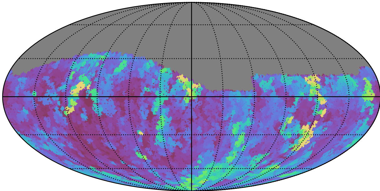
too_100_1v3.4_10yrs Yr 1 g band: Max seeingEff
