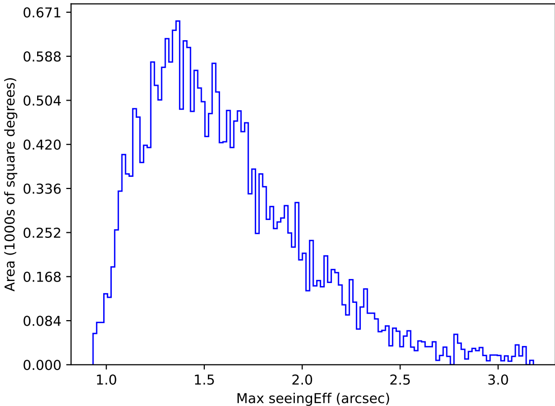
too_100_1v3.4_10yrs Yr 1 g band: Max seeingEff
