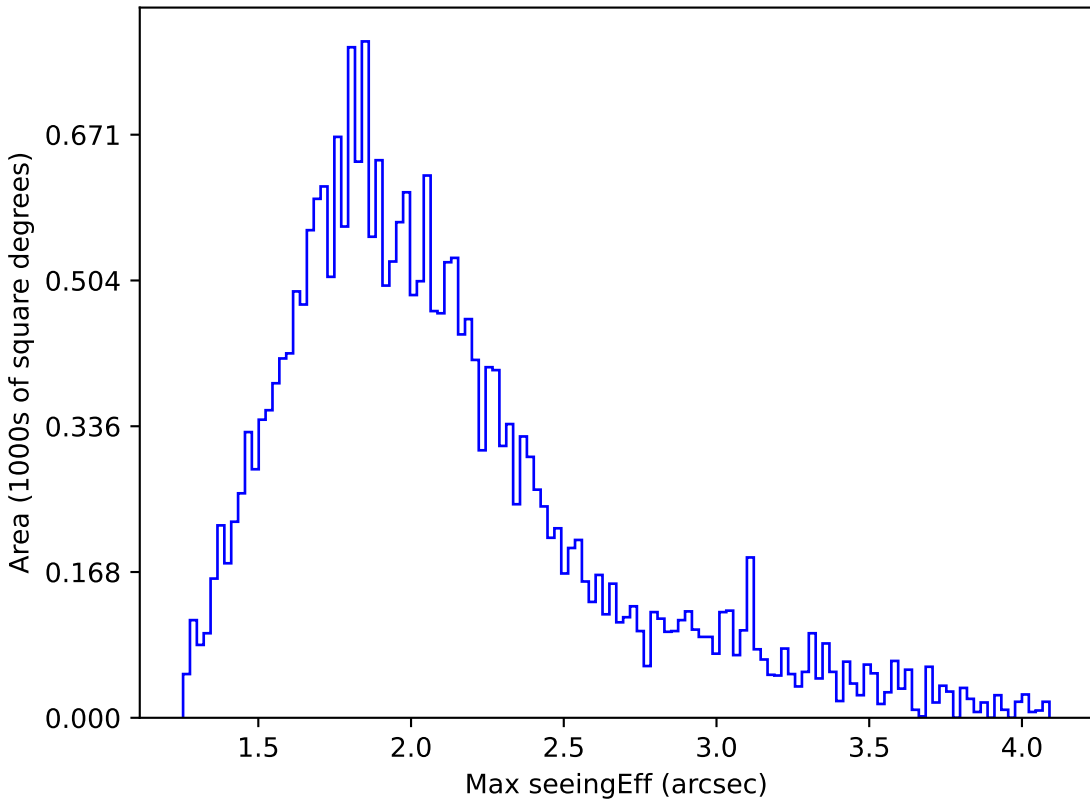
too_100_1v3.4_10yrs Yr 1 all bands: Max seeingEff
