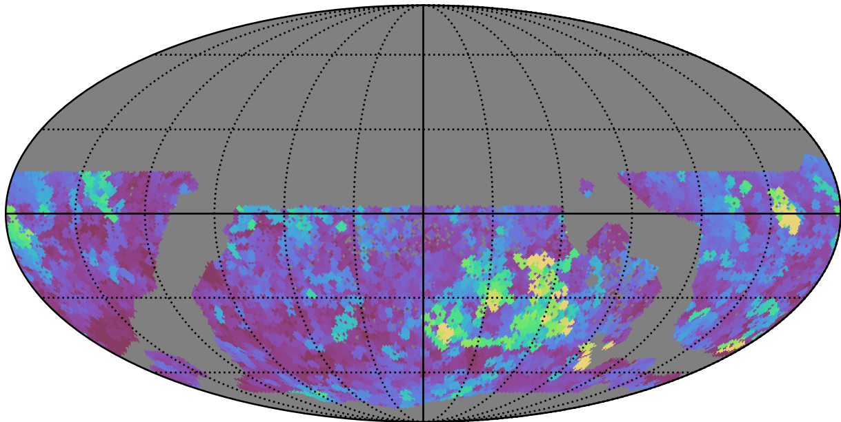
too_100_1v3.4_10yrs WFD z band: Max seeingEff
