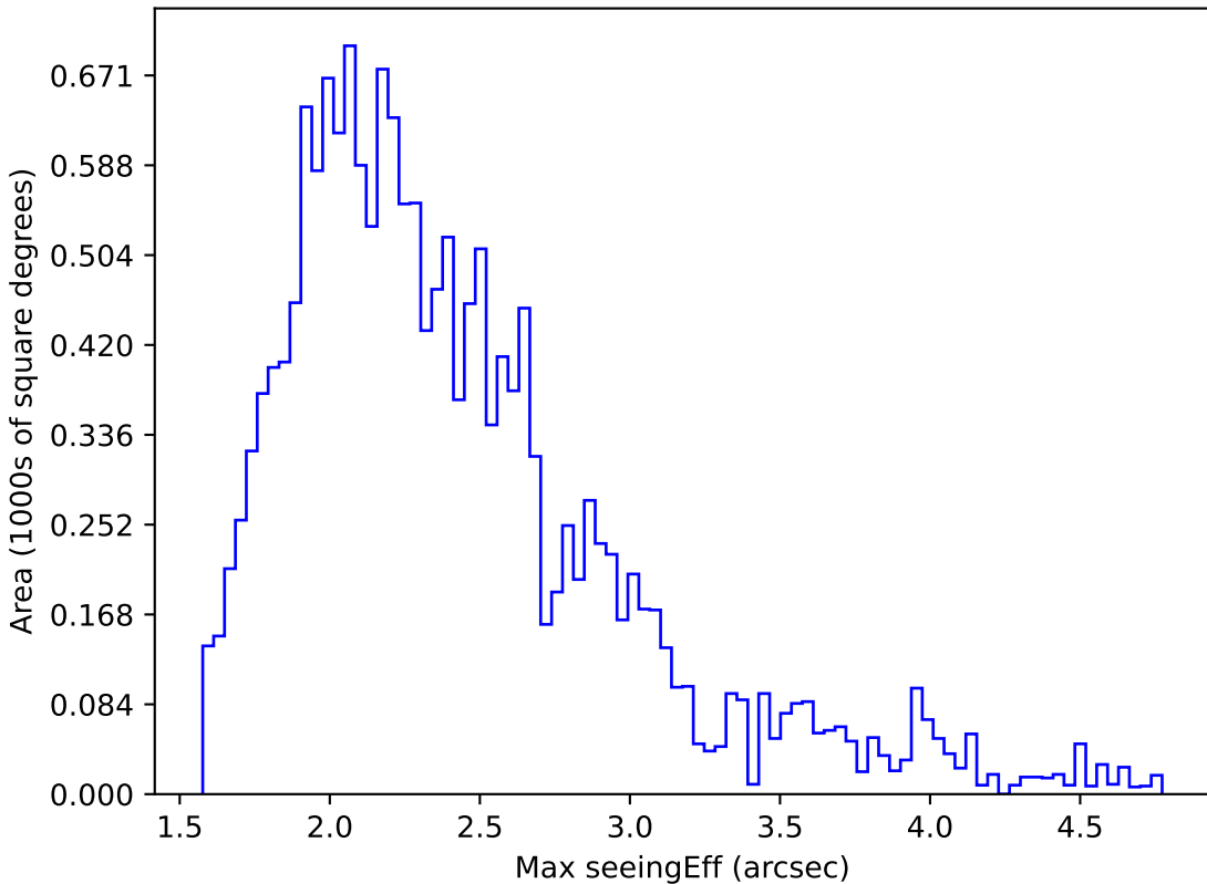
too_100_1v3.4_10yrs WFD y band: Max seeingEff
