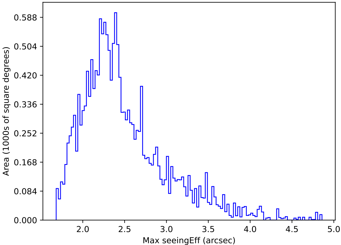
too_100_1v3.4_10yrs WFD u band: Max seeingEff
