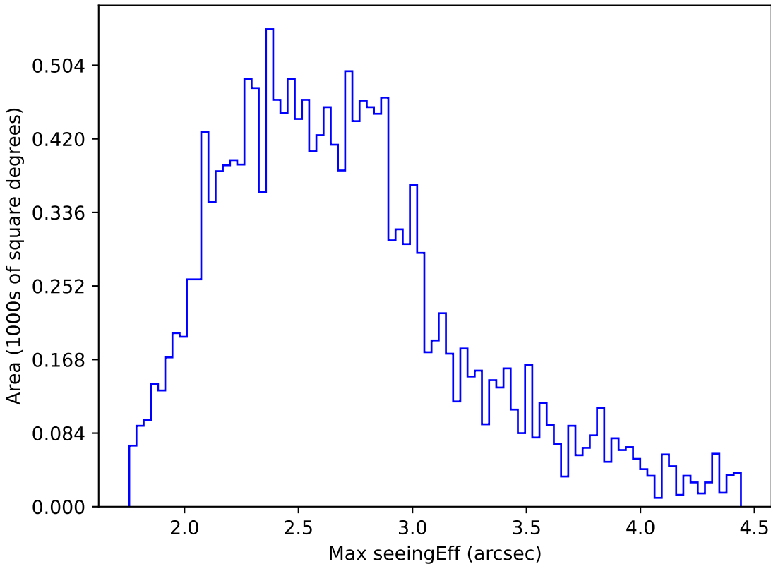
too_100_1v3.4_10yrs WFD r band: Max seeingEff
