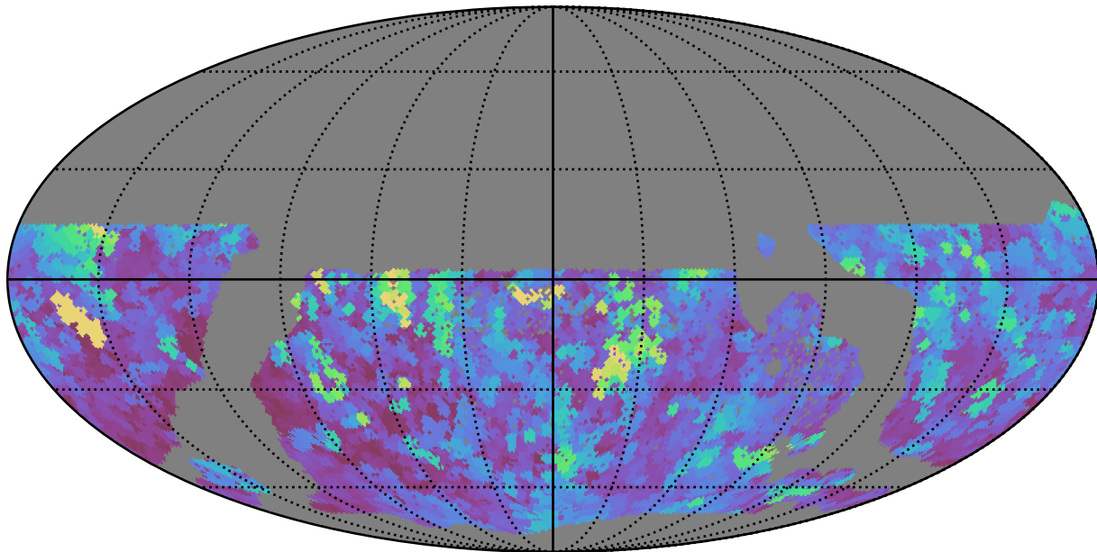
too_100_1v3.4_10yrs WFD i band: Max seeingEff
