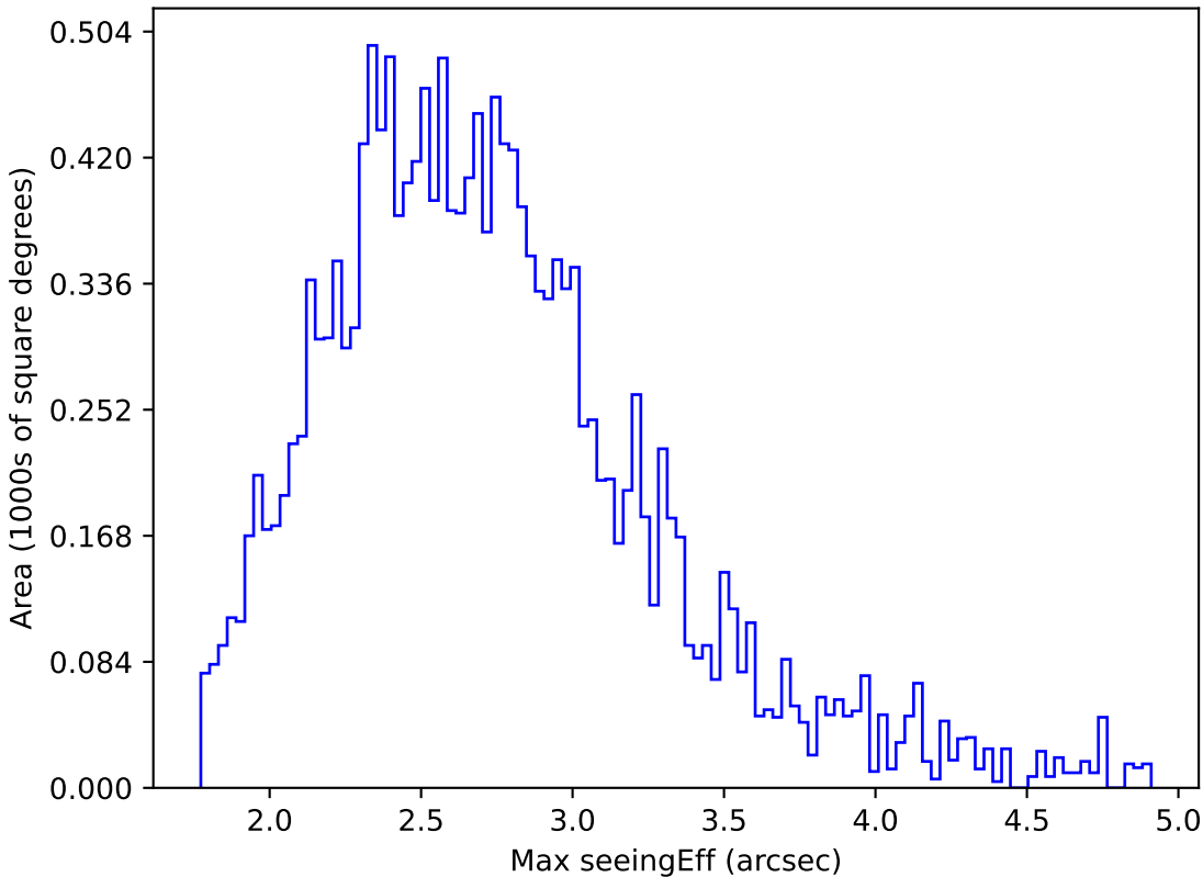
too_100_1v3.4_10yrs WFD i band: Max seeingEff
