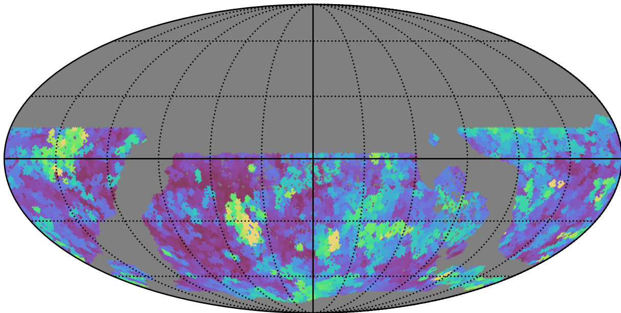
too_100_1v3.4_10yrs WFD g band: Max seeingEff
