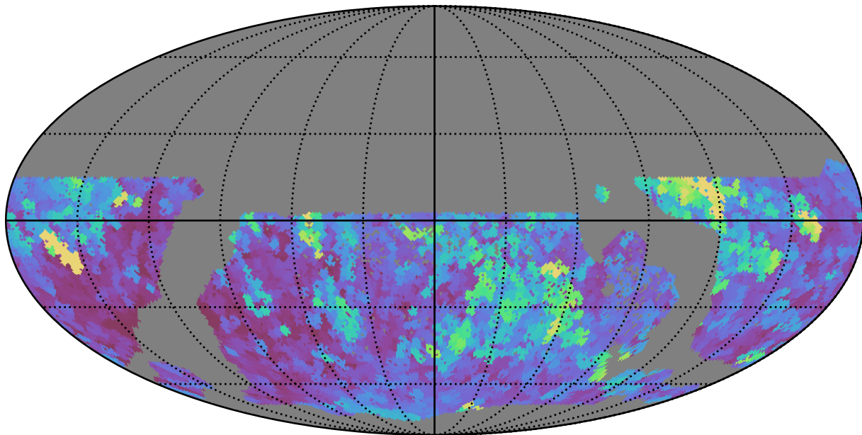
too_100_1v3.4_10yrs WFD all bands: Max seeingEff
