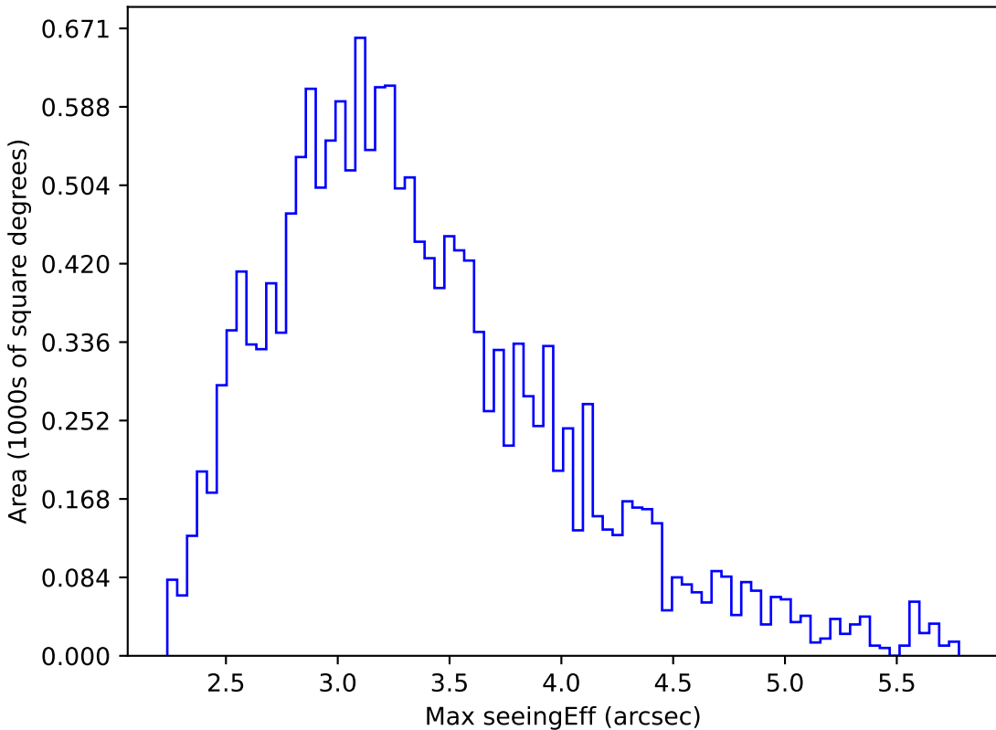
too_100_1v3.4_10yrs WFD all bands: Max seeingEff
