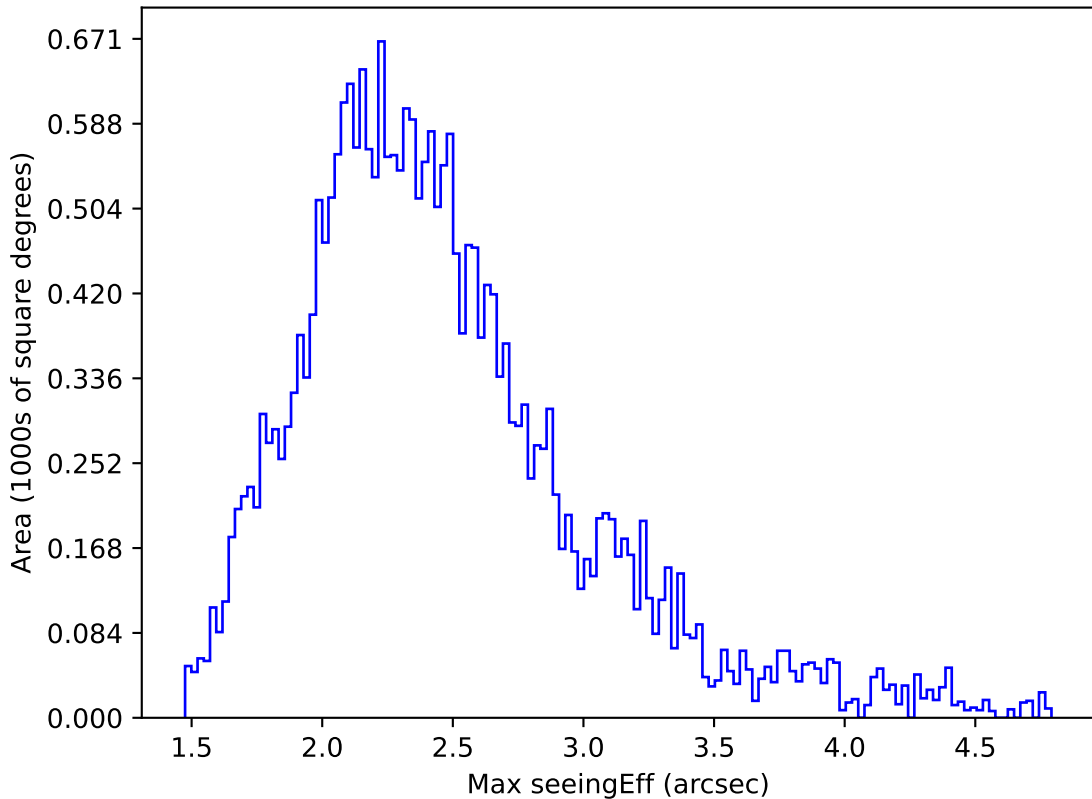
too_100_1v3.4_10yrs All sky z band: Max seeingEff
