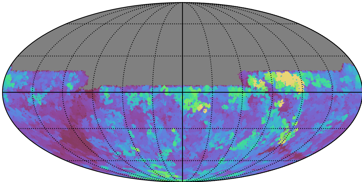
too_100_1v3.4_10yrs All sky u band: Max seeingEff
