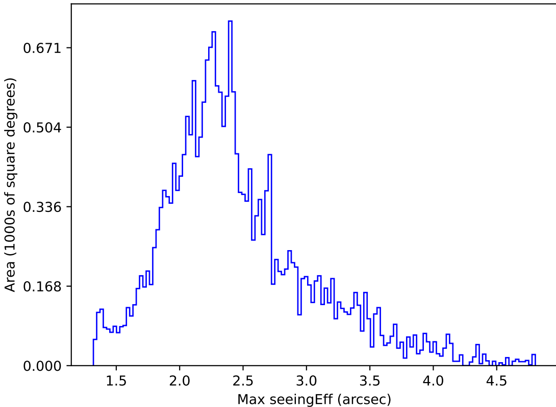
too_100_1v3.4_10yrs All sky u band: Max seeingEff
