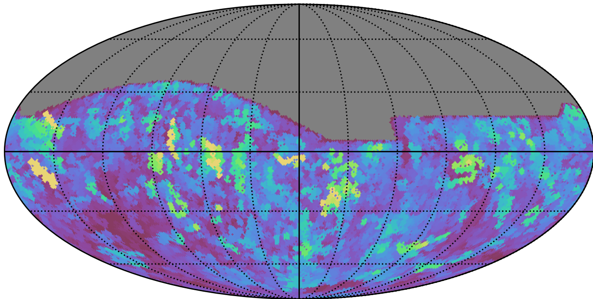
too_100_1v3.4_10yrs All sky i band: Max seeingEff
