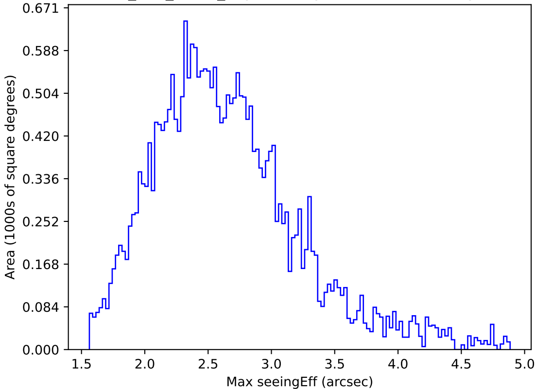
too_100_1v3.4_10yrs All sky i band: Max seeingEff
