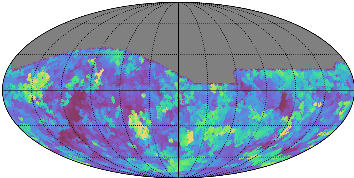
too_100_1v3.4_10yrs All sky g band: Max seeingEff
