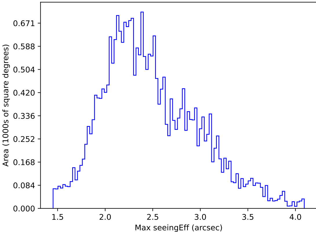
too_100_1v3.4_10yrs All sky g band: Max seeingEff
