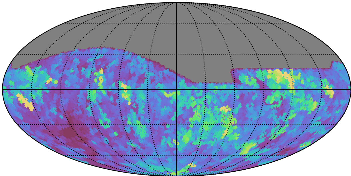
too_100_1v3.4_10yrs All sky all bands: Max seeingEff
