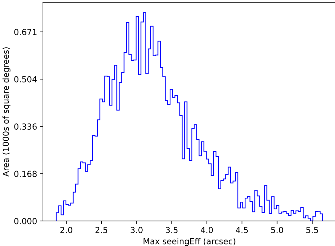
too_100_1v3.4_10yrs All sky all bands: Max seeingEff
