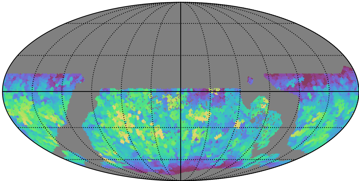
too_100_1v3.4_10yrs WFD z band: Max saturation_mag
