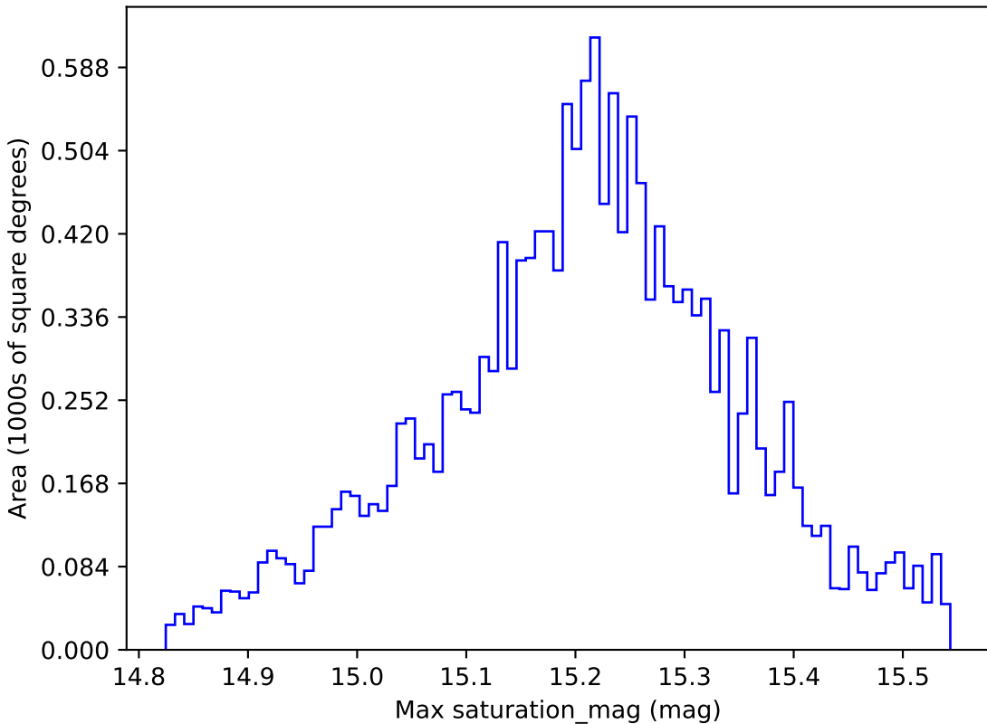
too_100_1v3.4_10yrs WFD z band: Max saturation_mag
