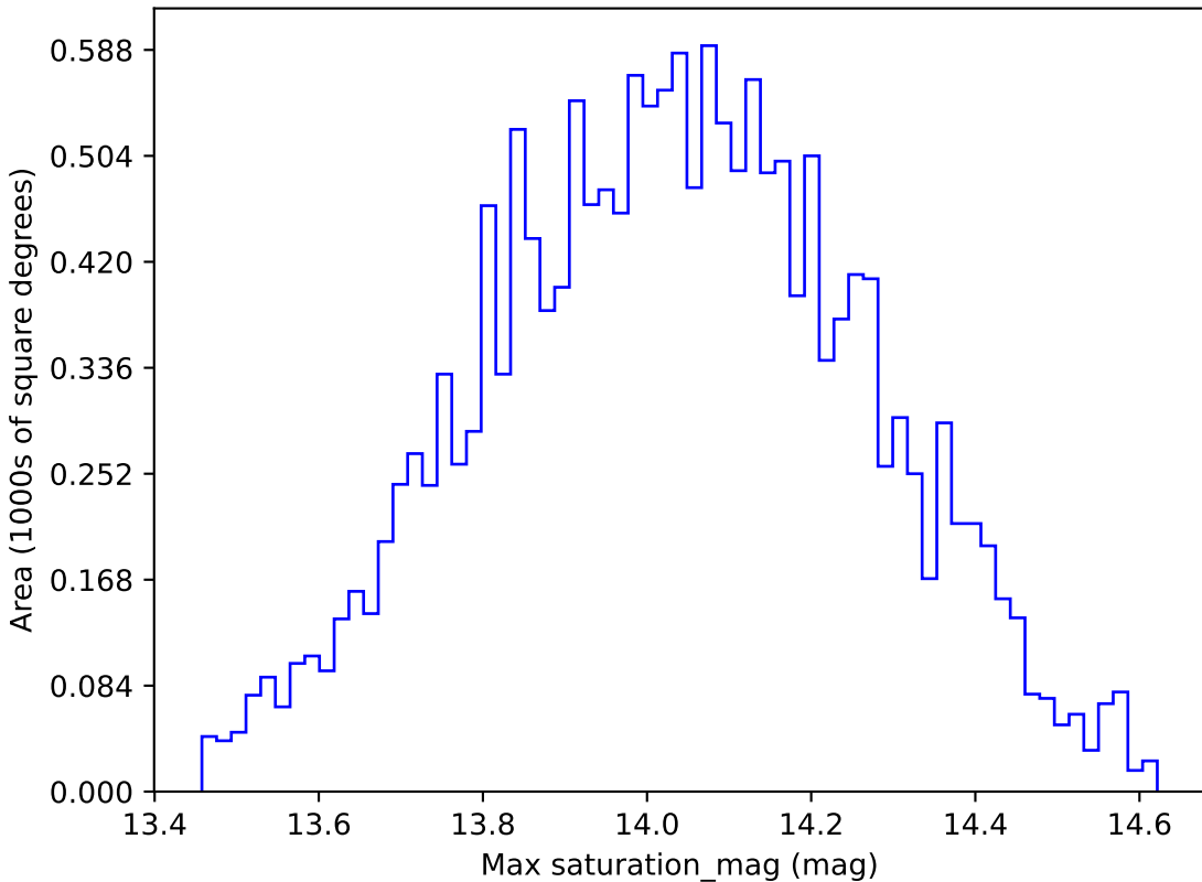
too_100_1v3.4_10yrs WFD u band: Max saturation_mag
