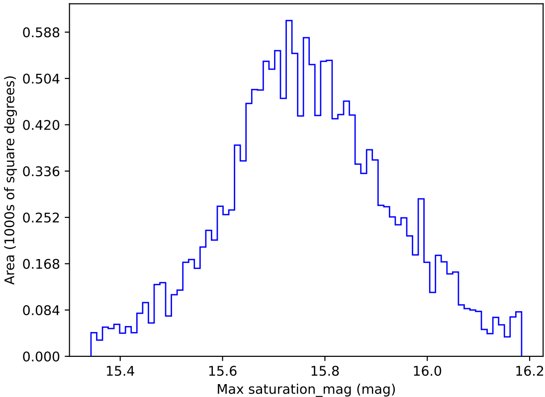
too_100_1v3.4_10yrs WFD r band: Max saturation_mag
